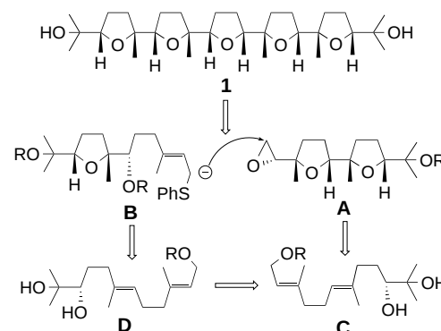
Scheme 1. Retrosynthetic analysis of the reported glabrescol ( 1 ).
